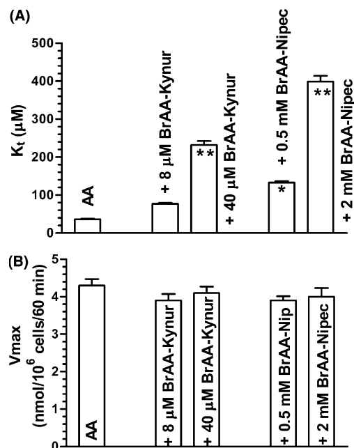
Figure 3. K_t and V_{\max} values of AA transport obtained in the absence and in the presence of increasing concentrations of the BrAA conjugates of nipecotic and kynurenic acids. The reference values for AA alone are K_t = 36 \pm 3 \mu\text{M} and V_{\max} = 4.3 \pm 0.3 \text{ nmol}/10^6 \text{ cells} . ^{*}p < 0.05 , ^{**}p < 0.001 significant versus [ ^{14}\text{C} ]AA alone.
