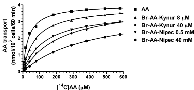
Figure 2. Kinetics of AA uptake in HRPE and inhibition of this transport by different concentrations of BrAA conjugates of nipecotic and kynurenic acids. These are single representative experiments performed in duplicate.
