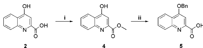
Scheme 1. Reagents and conditions: (i) \text{H}_2\text{SO}_4 96%, anhydrous MeOH, reflux; (ii) (a) benzylbromide, \text{K}_2\text{CO}_3 , anhydrous DMF, (b) NaOH, \text{H}_2\text{O}/\text{MeOH} (1:1).
