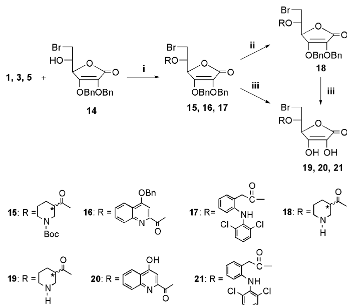
Scheme 3. Reagents and conditions: (i) DMAP, DCC, anhydrous \text{CH}_2\text{Cl}_2 or \text{CH}_2\text{Cl}_2/\text{DMF} ; (ii) TFA, anhydrous \text{CH}_2\text{Cl}_2 ; (iii) \text{H}_2 , C/Pd 10%, \text{CH}_3\text{OH} .
