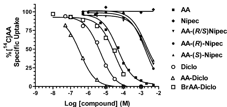
Figure 4. Inhibition of 50 \mu\text{M} [ ^{14}\text{C} ]AA uptake by AA, nipecotic and diclofenamic acids and their AA and BrAA-conjugates. These are single representative experiments performed in duplicate.
