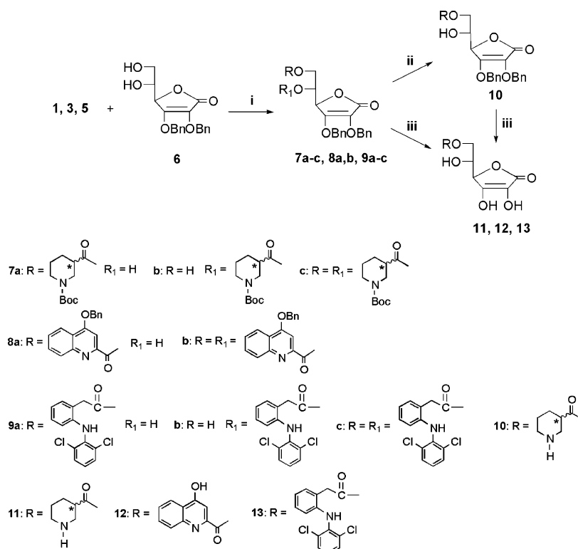
Scheme 2. Reagents and conditions: (i) DMAP, DCC, anhydrous \text{CH}_2\text{Cl}_2 or \text{CH}_2\text{Cl}_2/\text{DMF} ; (ii) TFA, anhydrous \text{CH}_2\text{Cl}_2 ; (iii) \text{H}_2 , C/Pd 10%, \text{CH}_3\text{OH} .
